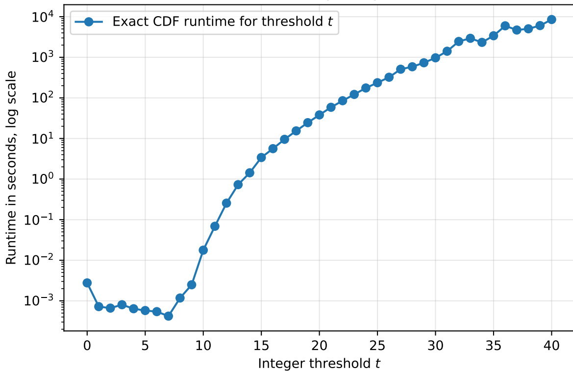
Exact CDF runtime by integer threshold
